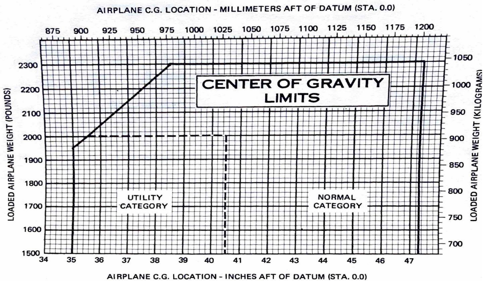
Figure 6-8. Center of Gravity Limits
